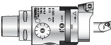
PSC40 - TRM50 Ø 2.5 ~ 108
