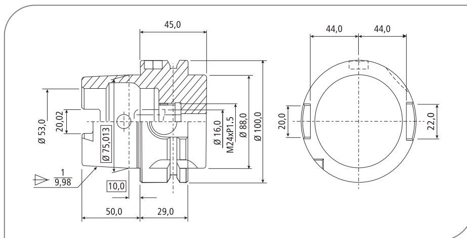
HSK - A100
