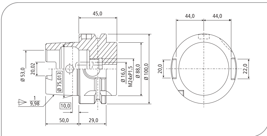
HSK - A100
