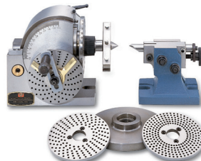
DIVISOR SEMI UNIVERSAL Modelo: BS-1
